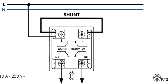
ROTARY SWITCH - 2 MODULES
