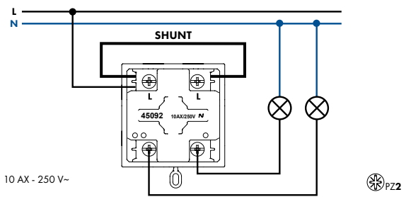
ROTARY 2-WAY SWITCH - 2 MODULES
